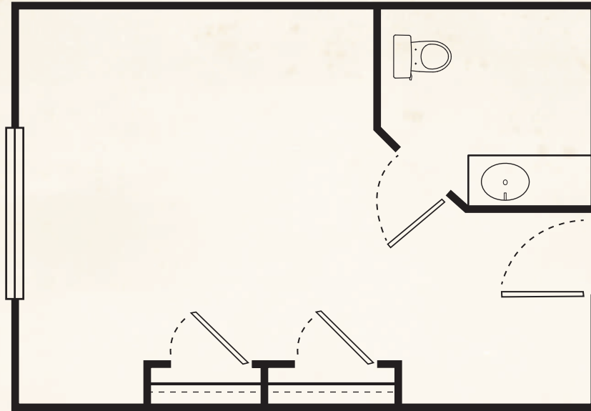
Style 1 336 Sq. Ft.
